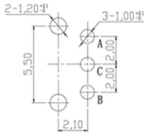
P. C. B Mounting Detail Viewed From Mounting Side
